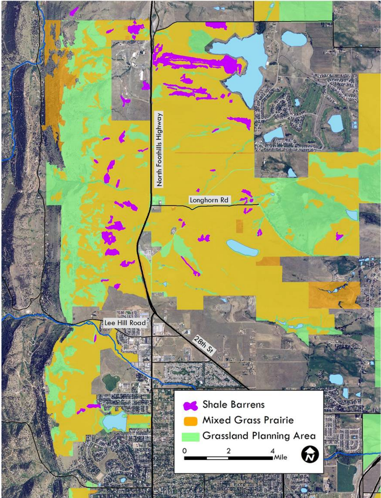
Figure 3: Distribution of Shale Barrens on Open Space and Mountain Parks
