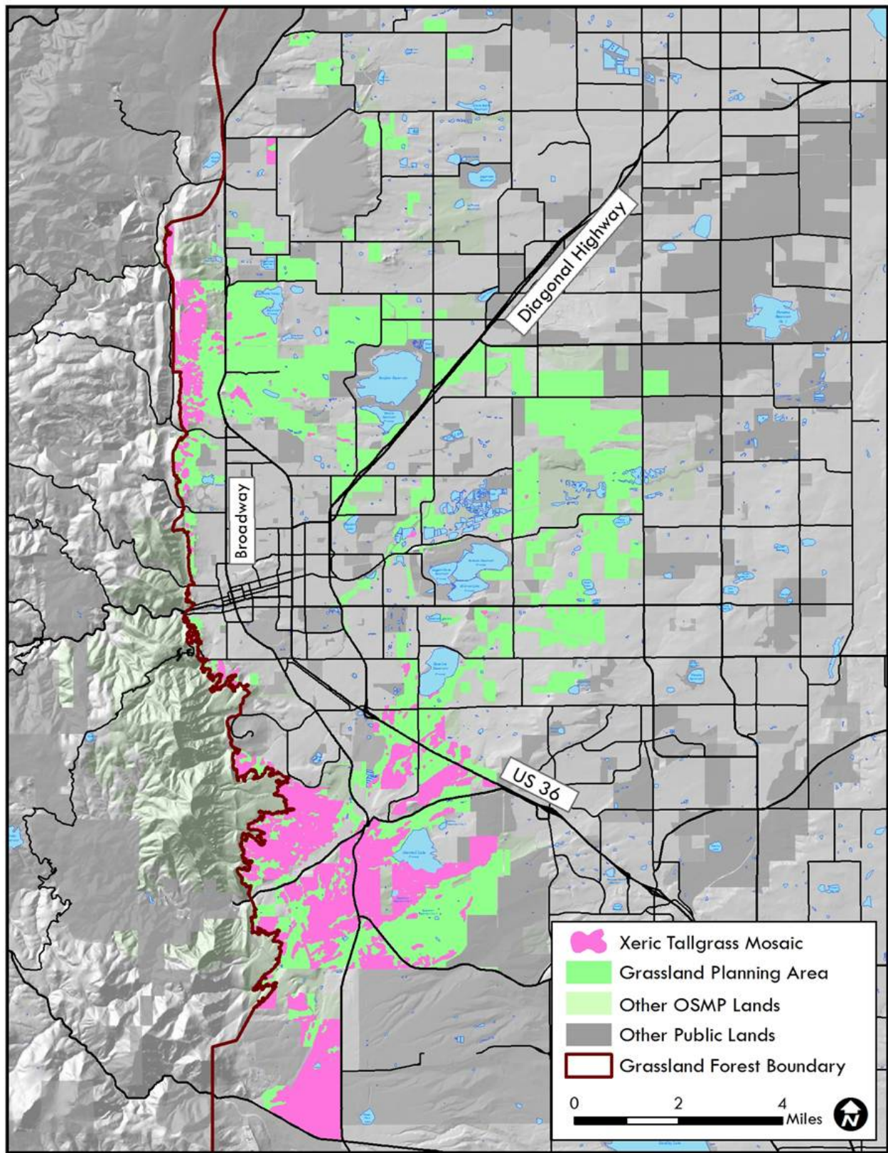
Figure 4: The Xeric Tallgrass Prairie in the Grassland Plan Planning Area
